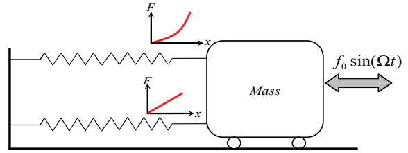
Fig. 3: Structural modeling of TLP considering hardening spring
