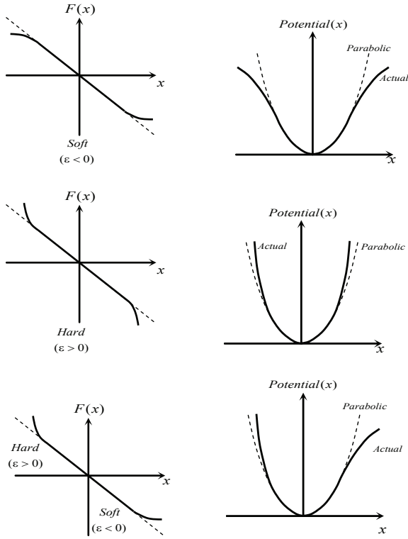
Fig. 5: power and potential figure for systems with large displacement
